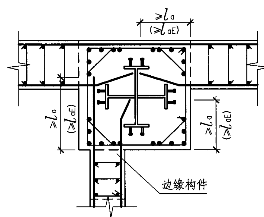
转角6
