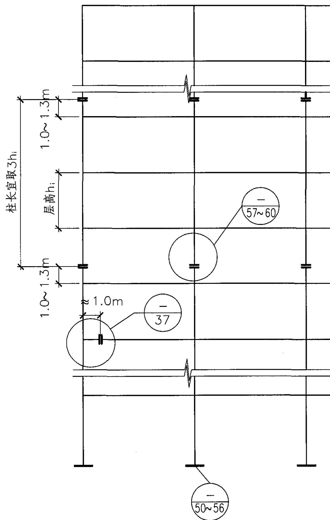
框架节点构造详图索引
